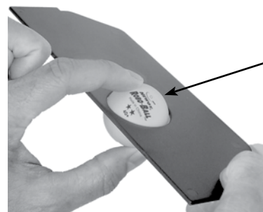
CHECKING BALL WITH BALL DAM (2055 ONLY)
